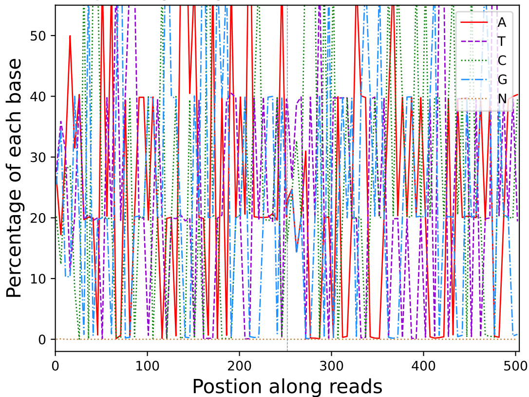
Base percentage along reads (R10211)
